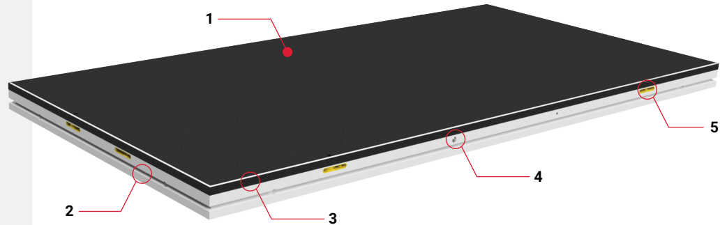
1 PLYWOOD TOP 2 HARDWARE SLOT 3 VELCRO ATTACHMENT 4 SPRING PIN LOCATOR 5 ROTARY LOCK
